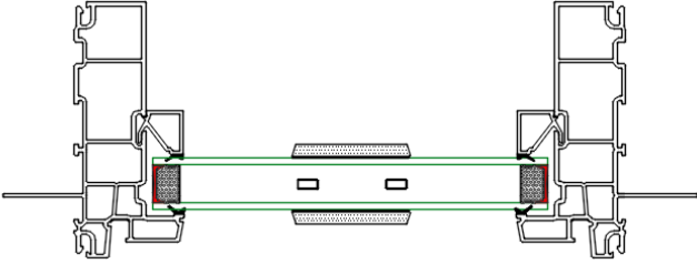
2" SDL PROFILE
