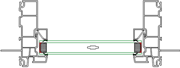
23/32" Contour In-Glass Grill
