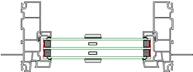
1" SDL PROFILE
