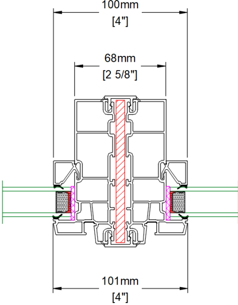
FLAT PLATE STEEL MULL
