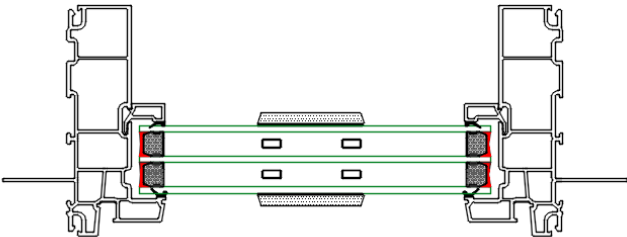
2" SDL PROFILE
