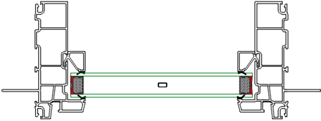
5/16" In-Glass Grill
