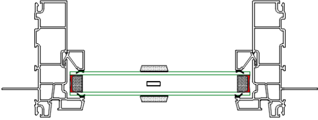
1" SDL PROFILE
