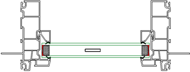
1" In-Glass Grill
