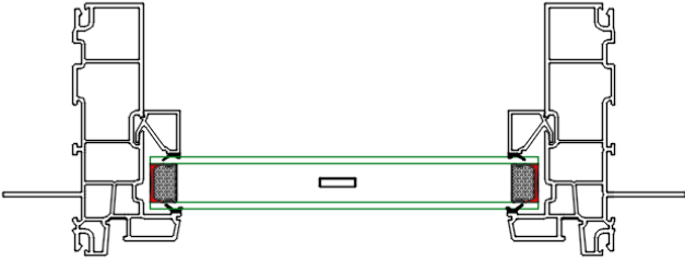
5/8" In-Glass Grill
